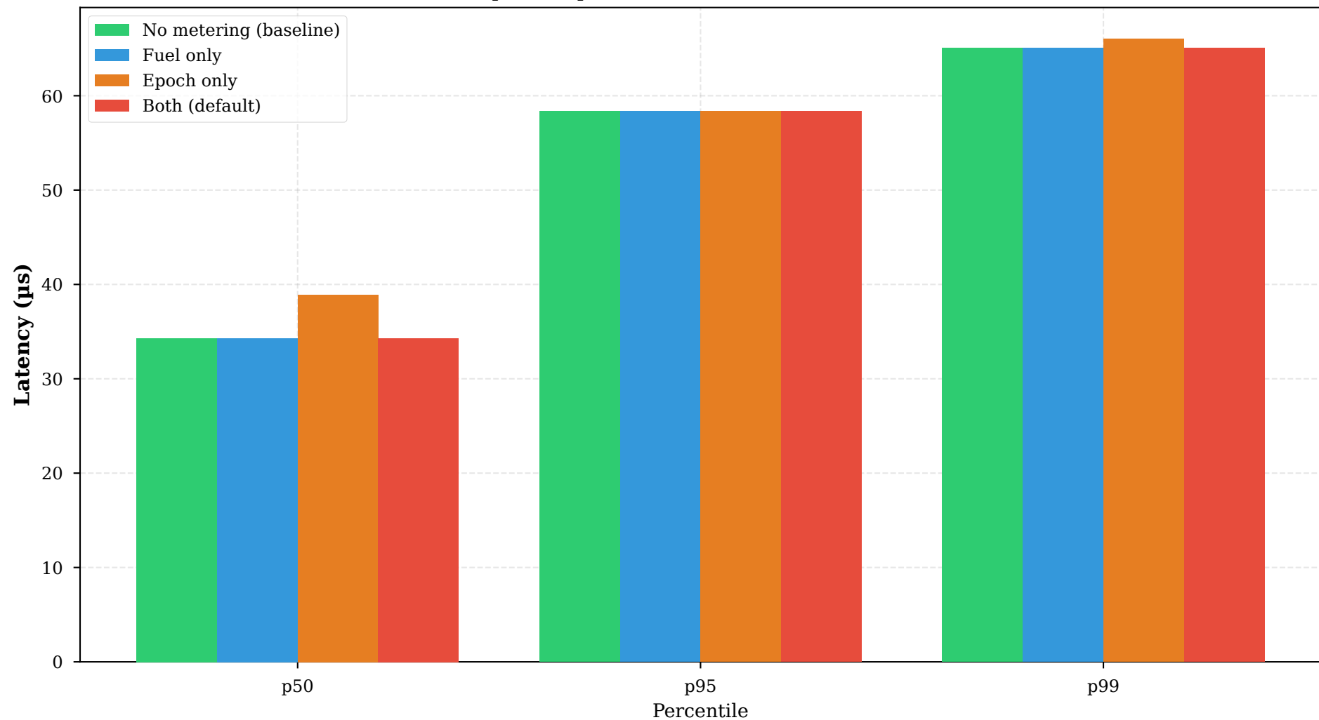
Figure 10: Metering overhead decomposition (shakedown-macos)
