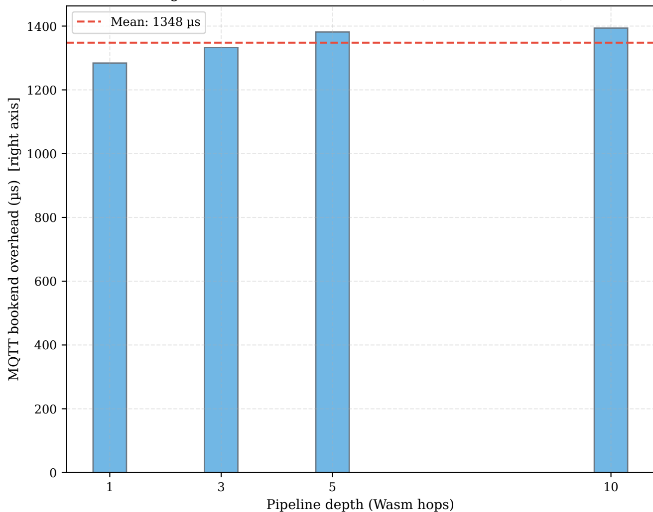
Figure 11b: Bookend cost isolation (shakedown-macos)
