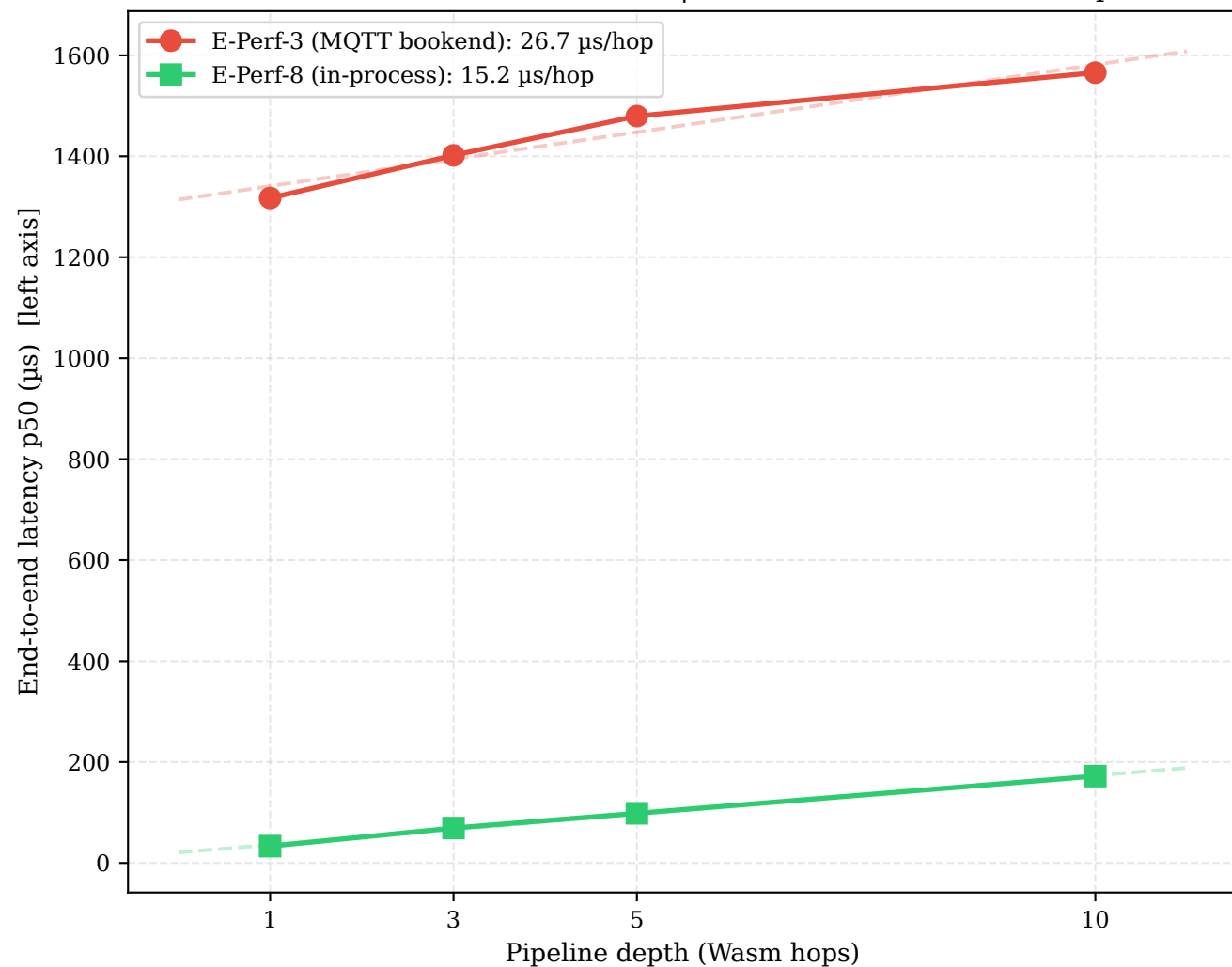
Figure 11a: Absolute latency (shakedown-macos)
