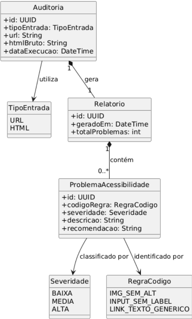
AccessAudit - Diagrama de Classes
