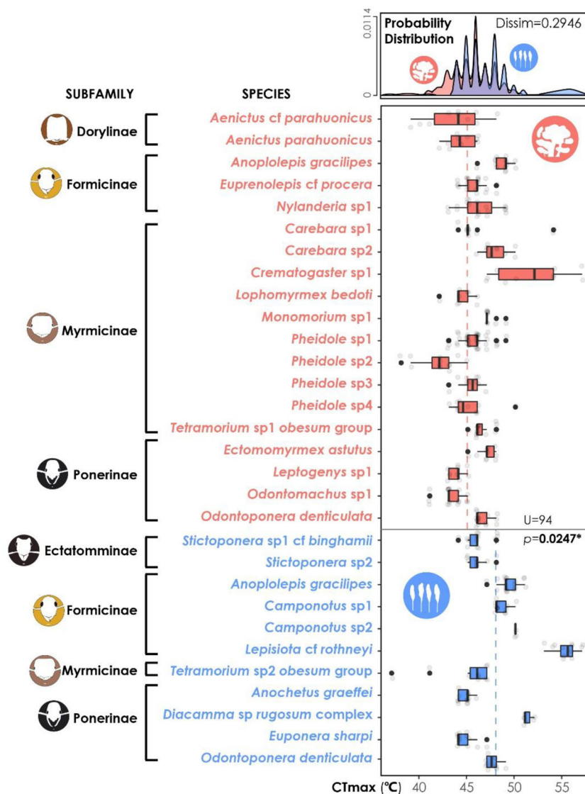
FIGURE 2 Top part: Trait probability density (TPD) incorporating intraspecific variation of critical thermal maximum ( CT_{max} ) in assemblage-level with presenting the TPD's dissimilarity (Dissim), and the purple colour represents the overlapped TPD between the forest and rubber plantation ant species. Lower part: CT_{max} of ant species from forest (red section) and rubber plantation (blue section) with p value of nonparametric Mann–Whitney U test of species average CT_{max} difference between the two habitats, and the dash lines indicate the mean value of CT_{max} across species in each habitat.
