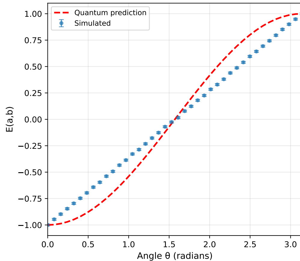
Quantum Measure
