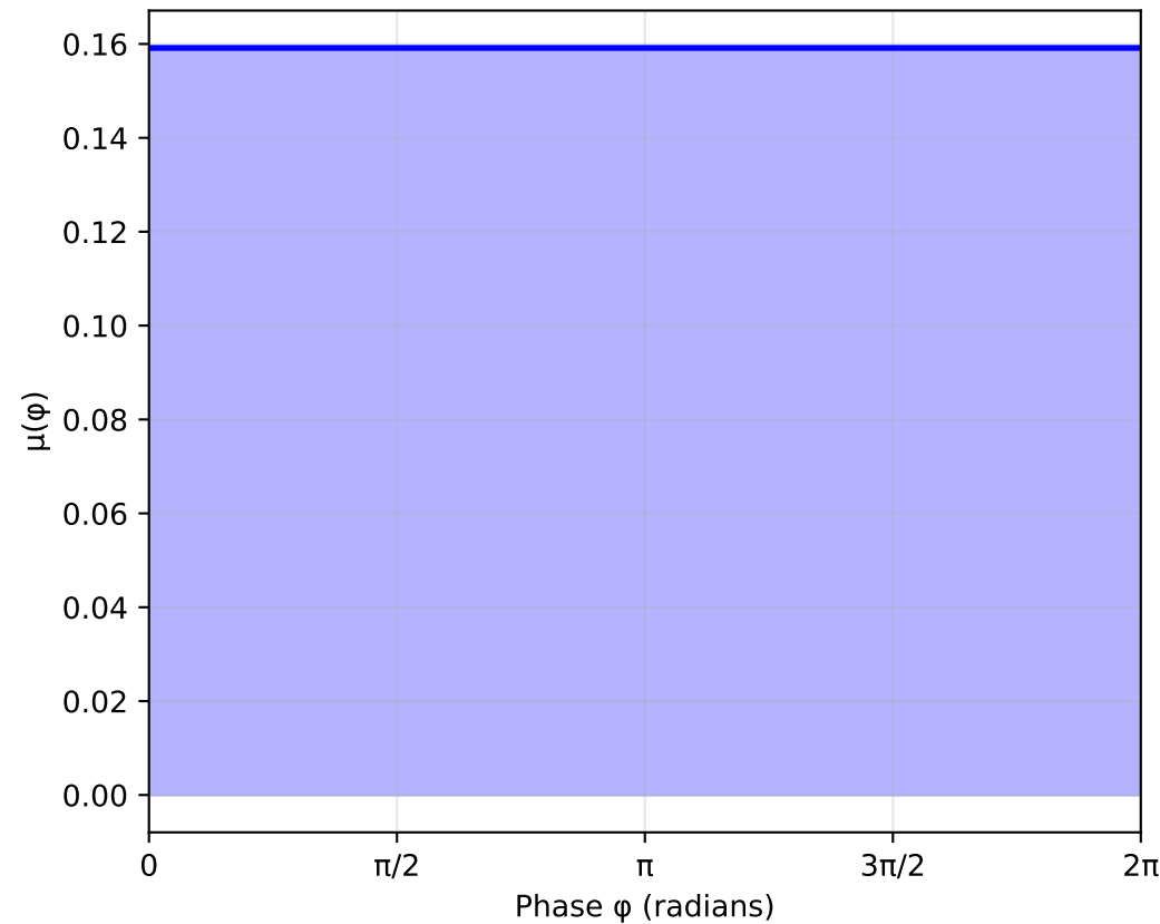
Quantum Measure (Uniform \rightarrow Born rule)
