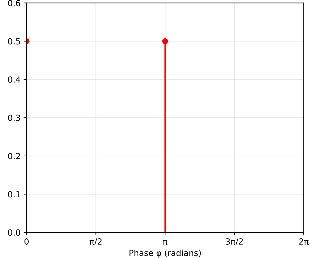
Bimodal Measure (Discrete: \delta(0) + \delta(\pi) )
