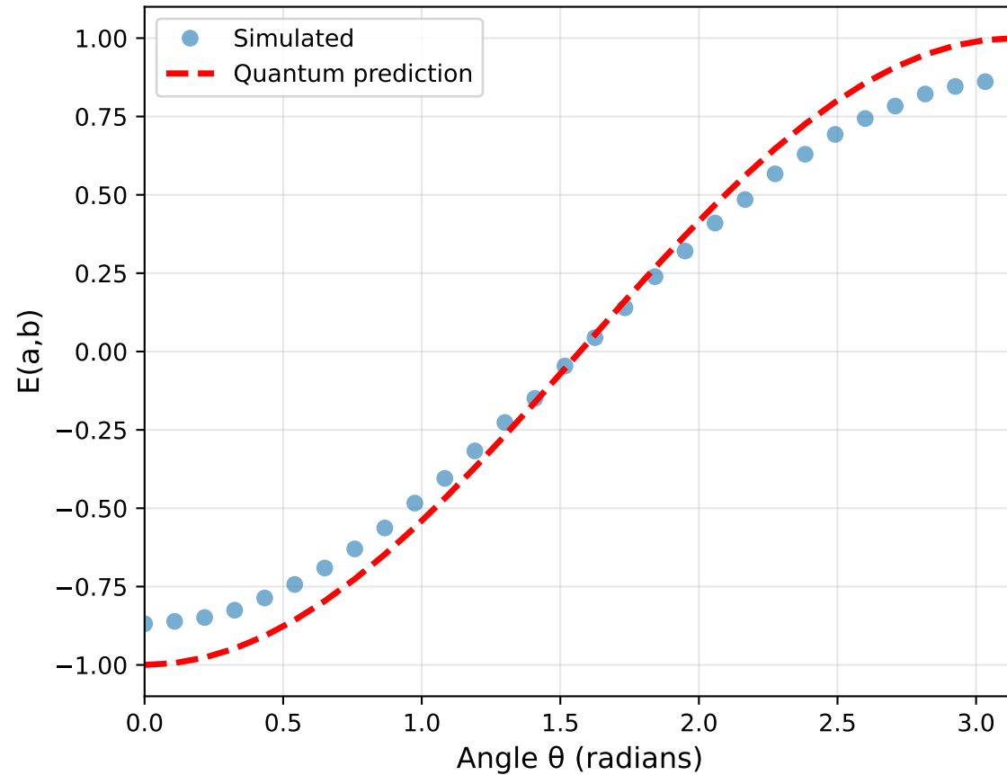
Peaked Measure
