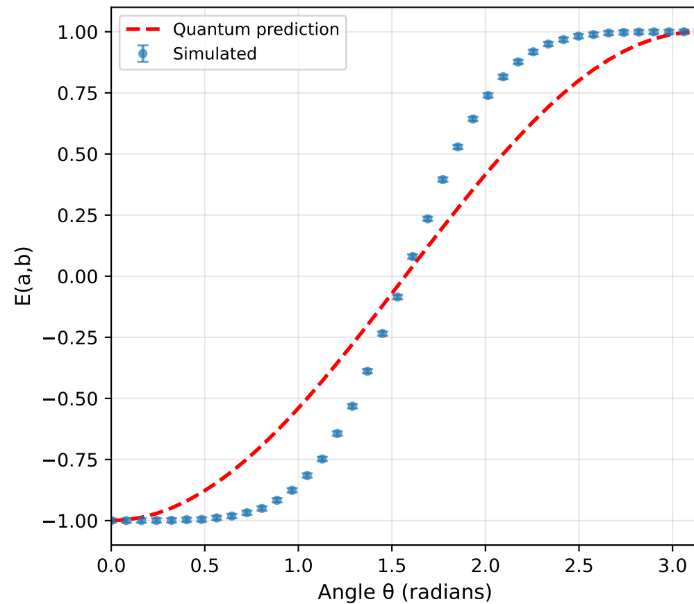
Peaked Measure
