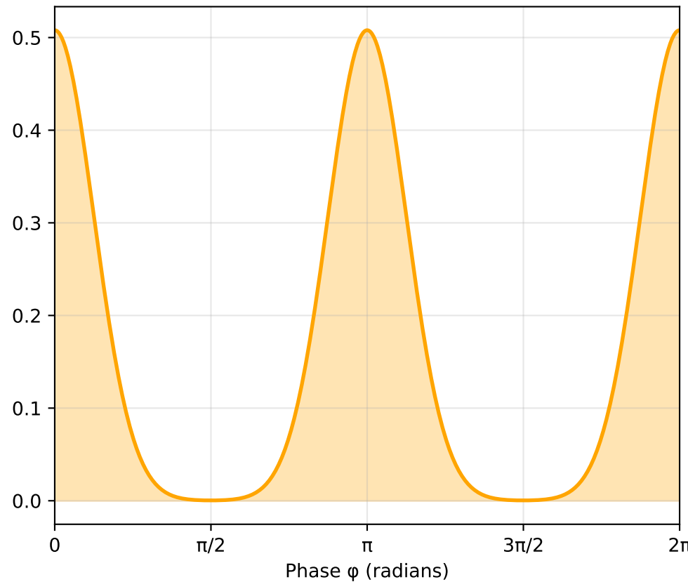
Peaked Measure (Concentrated at 0, \pi )
