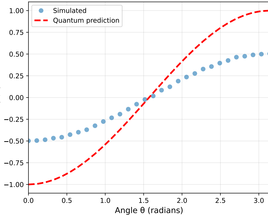
Quantum Measure
