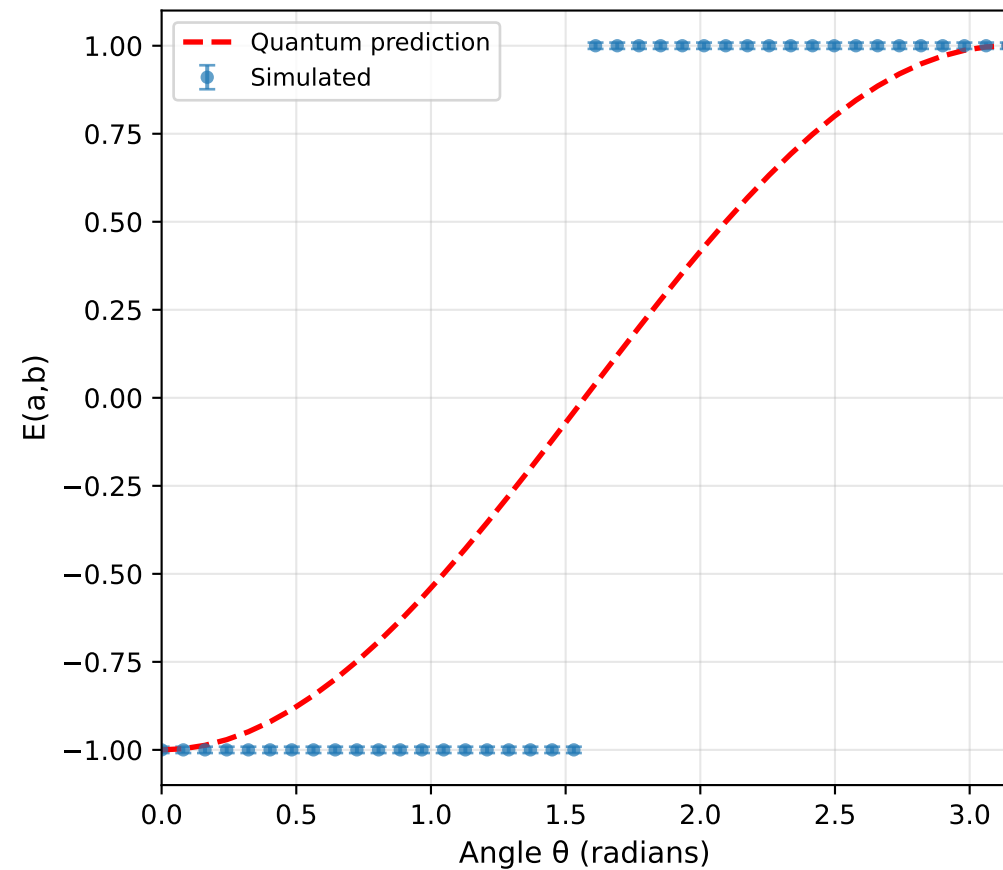
Bimodal Measure
