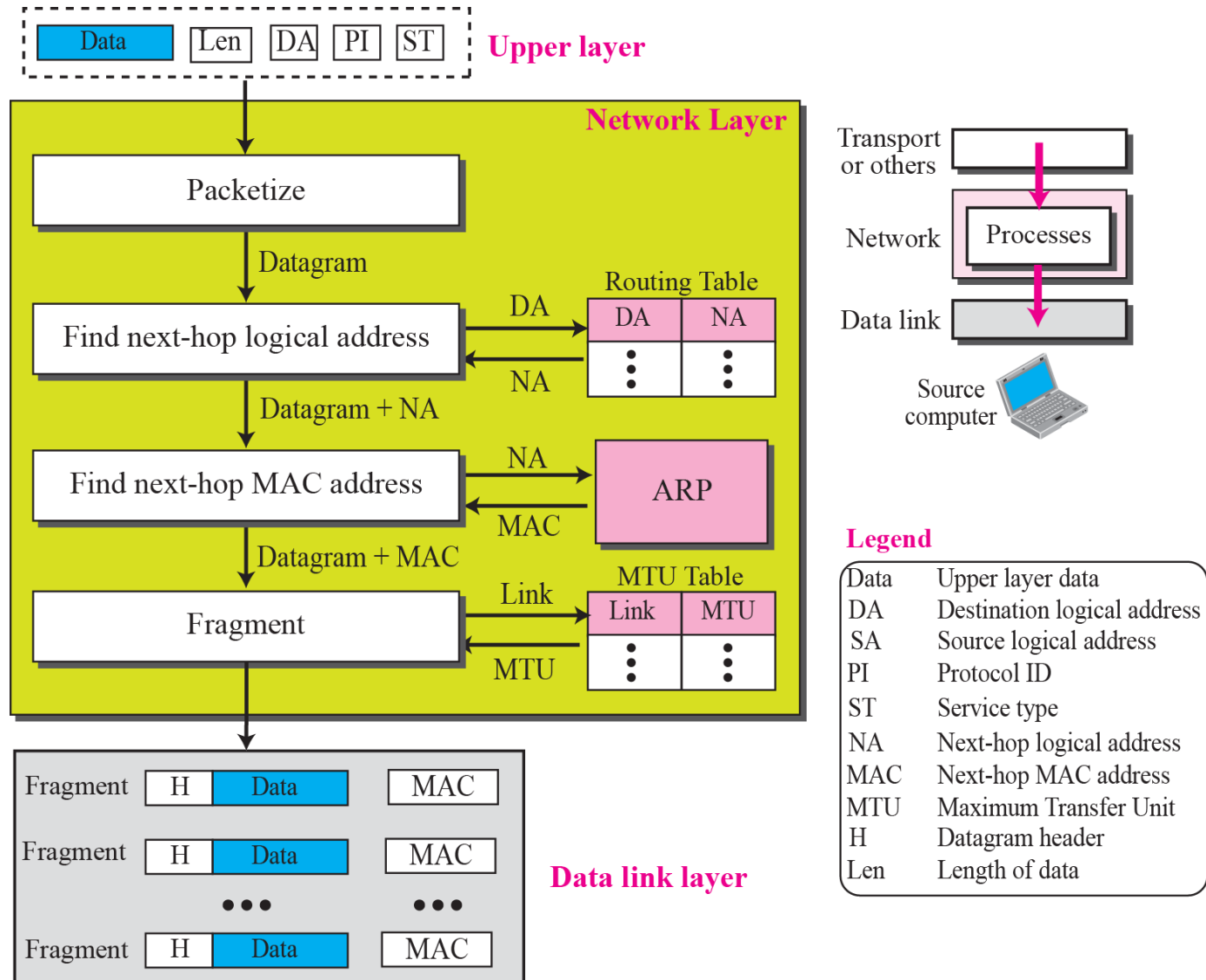
Figure 4.13 Services provided at the source computer
