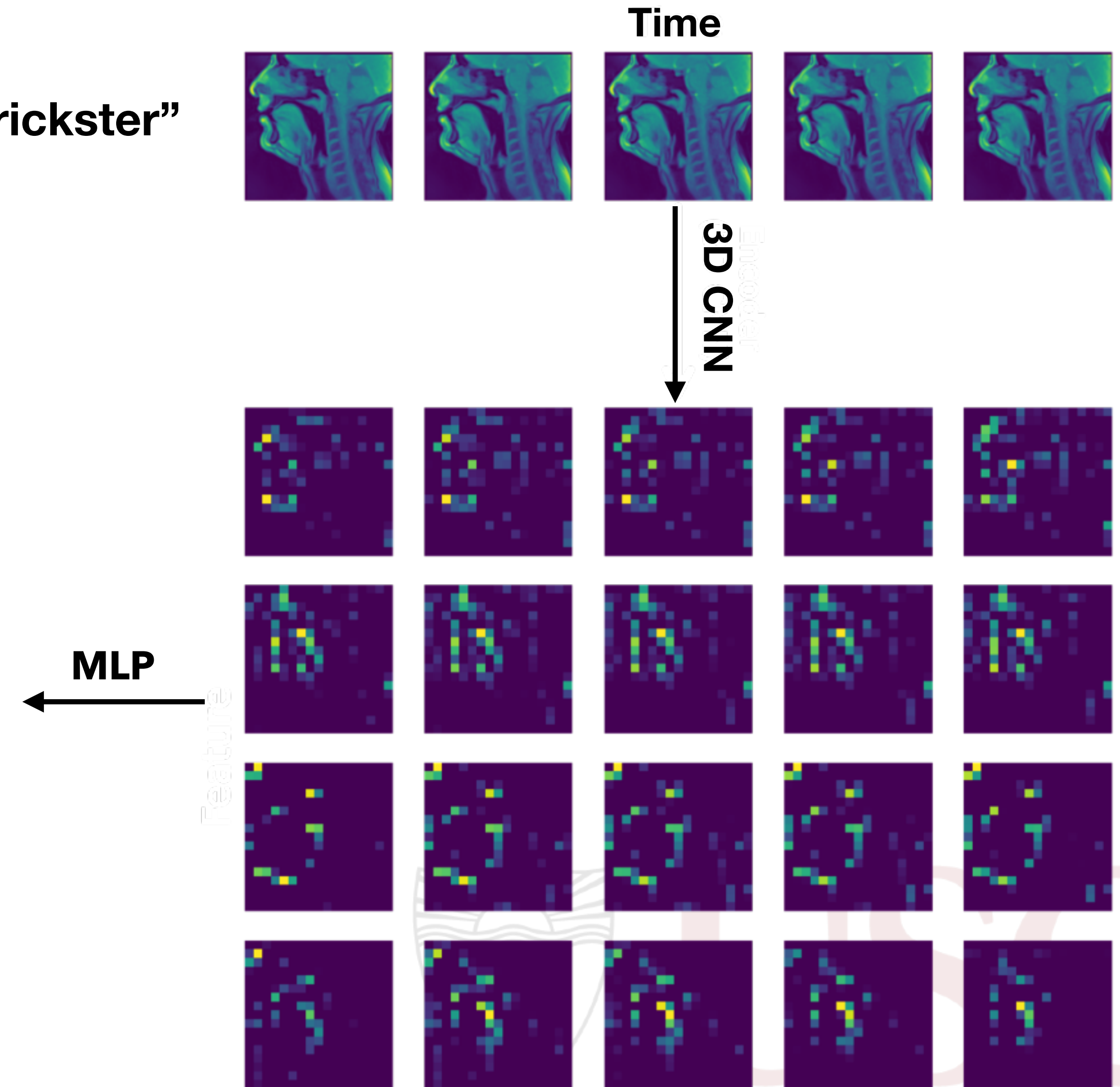
Latent dimensions (shown as saliency maps)
