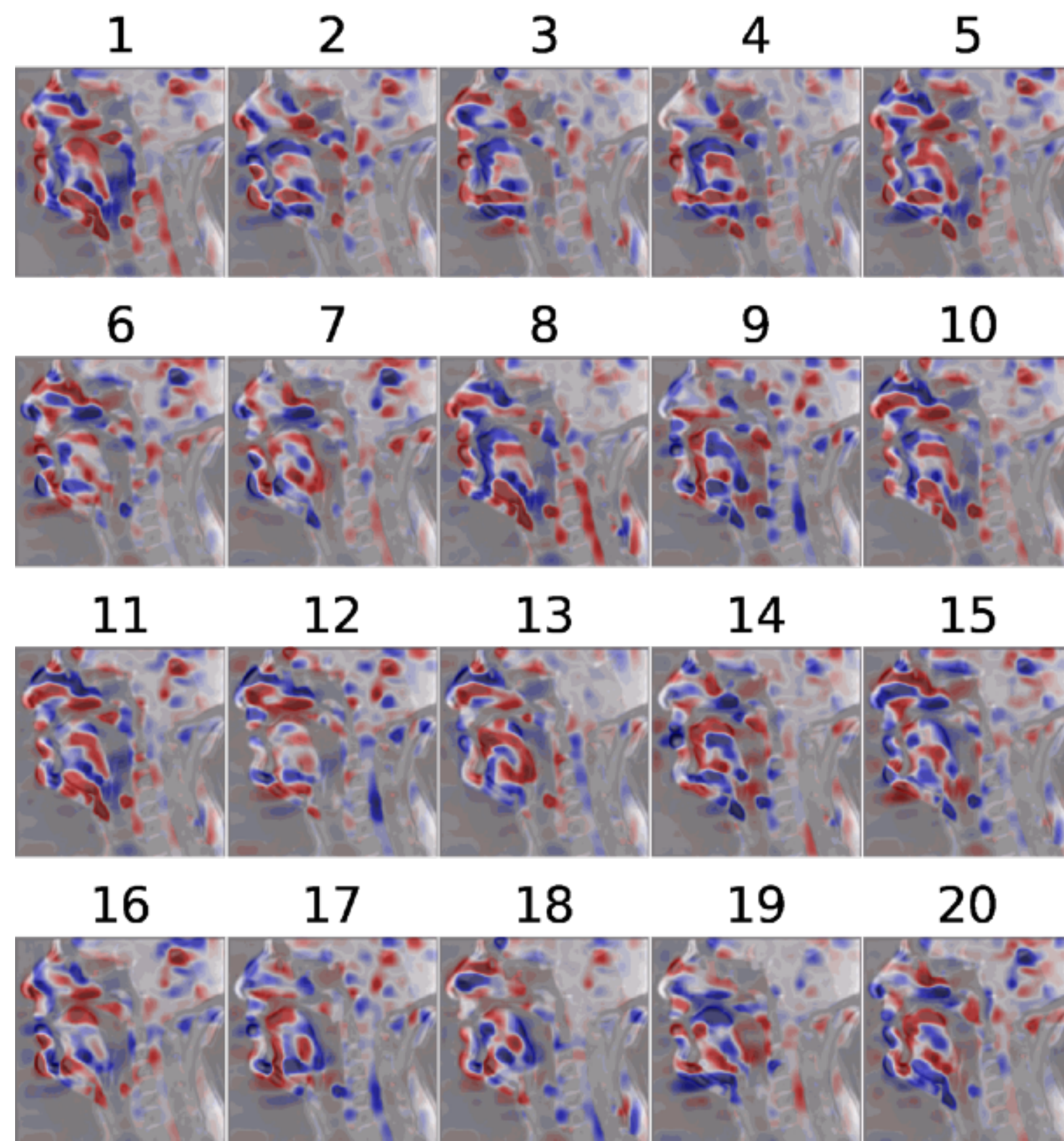
Latent dimensions (shown as saliency maps)
