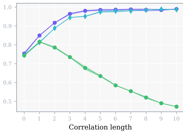
Softmax attention with MLP
