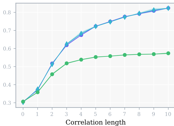
Full-Parameter linear attention
