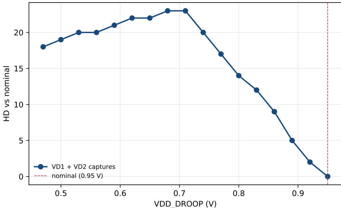
B-FE3 VD1 + VD2 Hamming response
