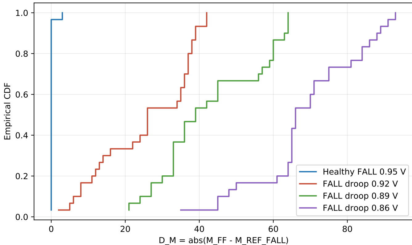
B-FE6-MARG0 M3 FALL distributions
