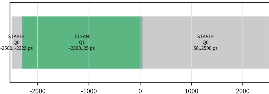
t0_5a_1p10_l2_long 1.10 V / L2 / 3002 ps
