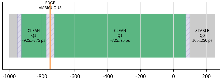
t0_5b_1p10_l1_recovery 1.10 V / L1 / 1502 ps
