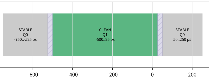
t0_5a_1p10_l2_boundary 1.10 V / L2 / 1190 ps
