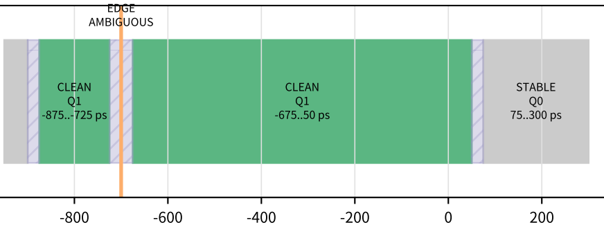
t0_5b_0p95_l3_recovery 0.95 V / L3 / 2002 ps
