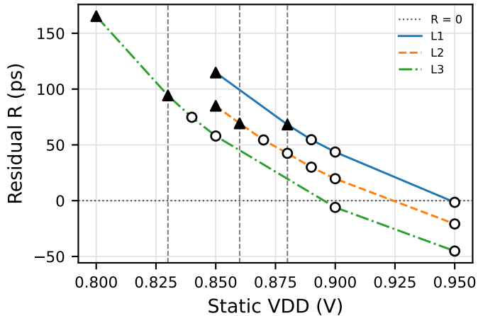
0.95 V baseline
