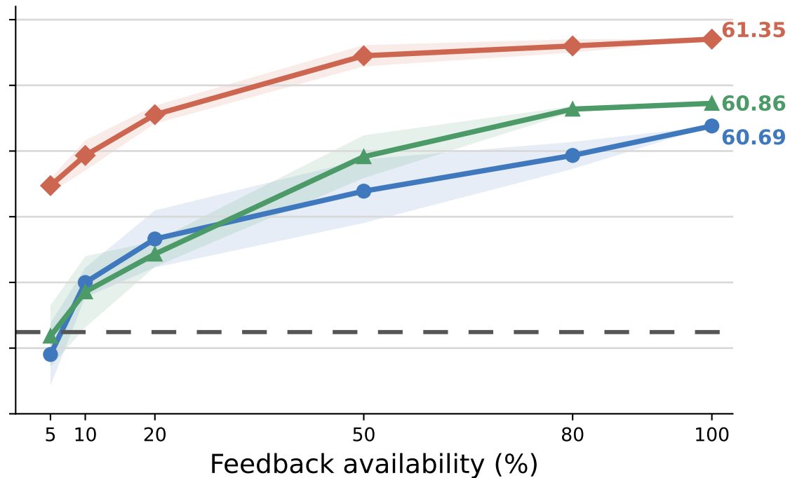
Qwen3.5-9B
