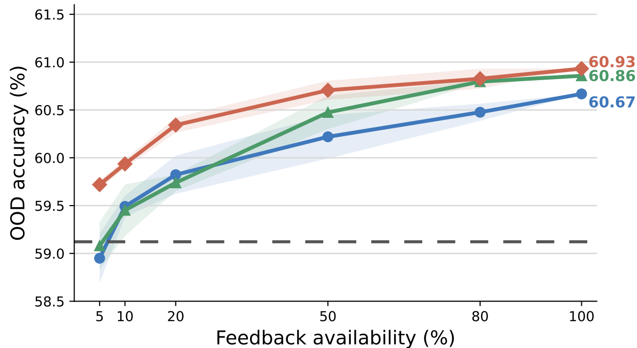
Qwen3.5-4B
