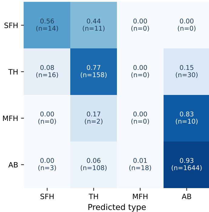
DINOv2 (frozen)
