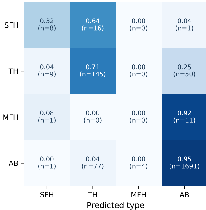
ResNet-50 (fine-tuned)
