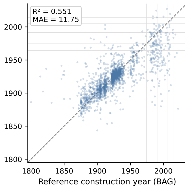
ResNet-50 (fine-tuned)
