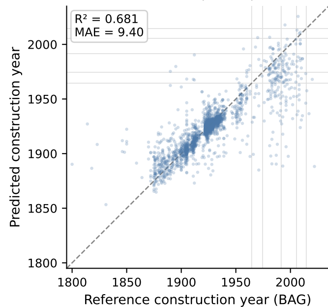
DINOv2 (frozen)
