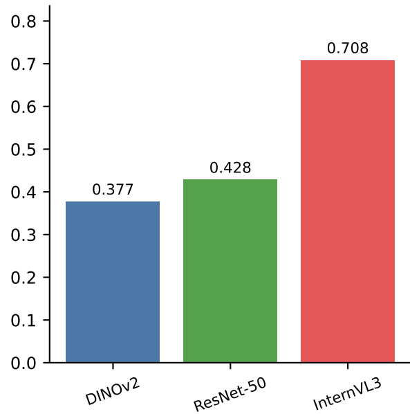
floors MAE ↓
