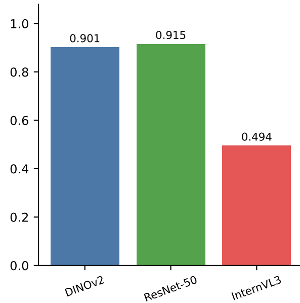
type accuracy
