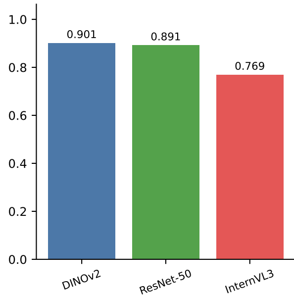
period accuracy
