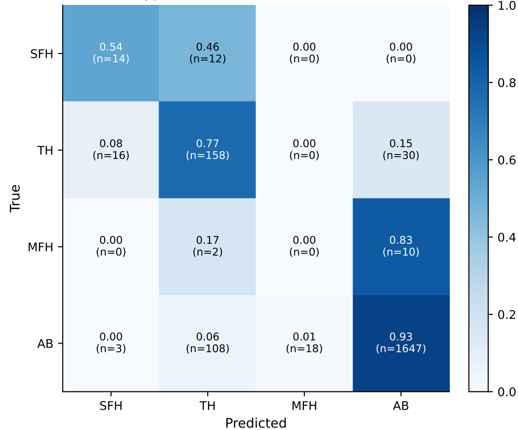
type confusion (row-normalized)
