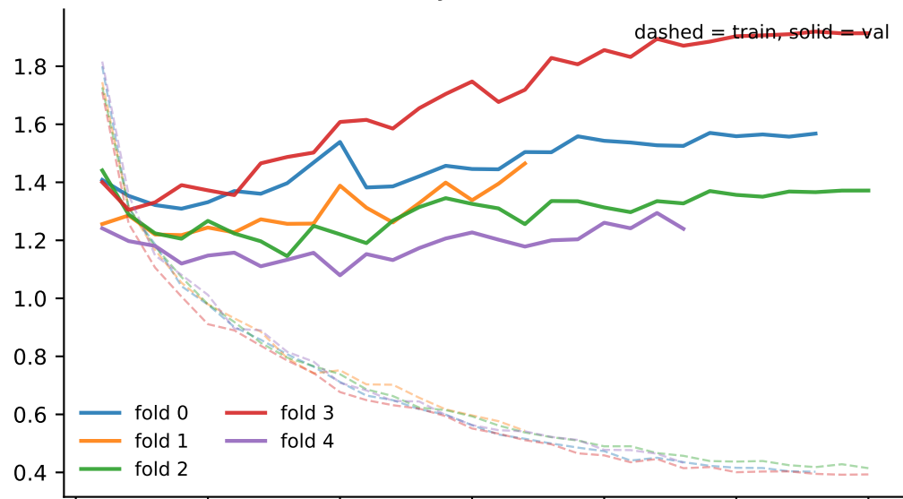
total loss (CE + year MSE + floors MSE)
