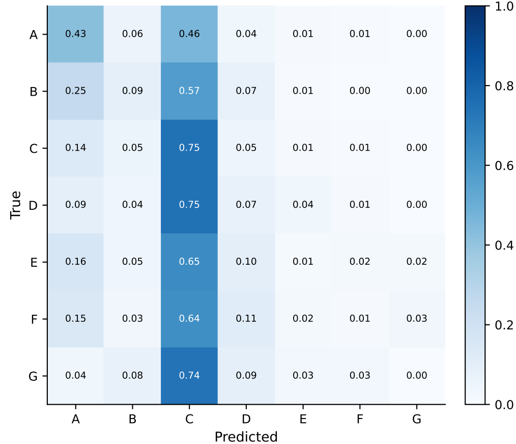
M1 (row-normalized)
