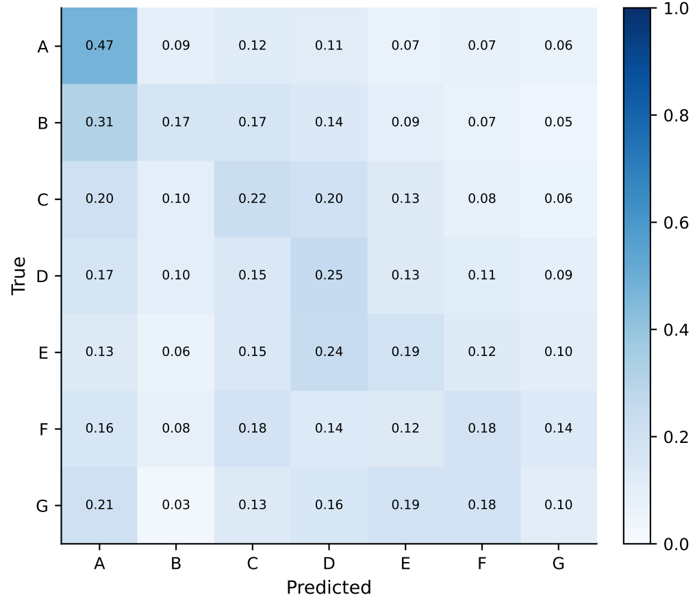
M2-DINOv2 (row-normalized)
