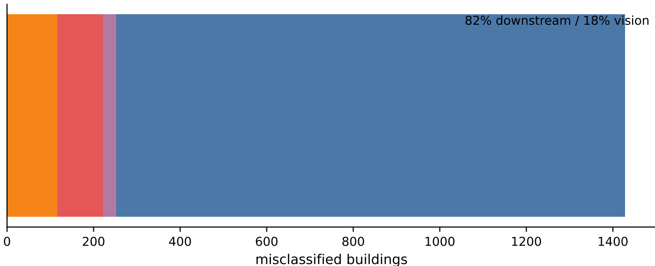
M3-DINOv2: error attribution (n_mis=1428)
