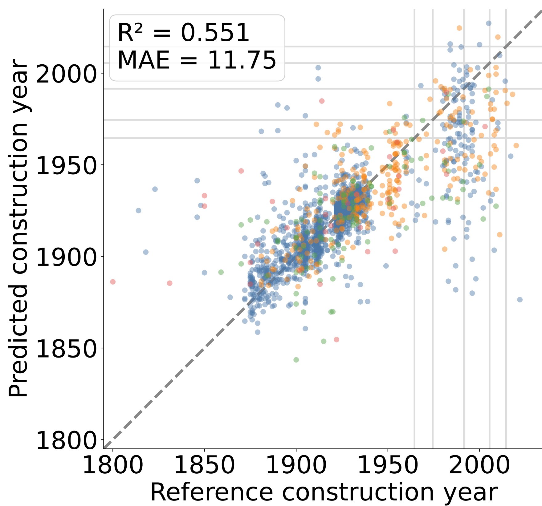
ResNet-50
