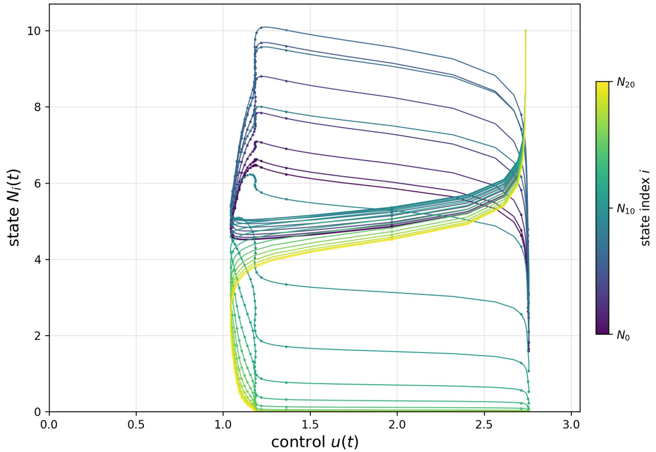
Figure 2. N(u) phase plot: each state component is plotted against the applied control; colors distinguish the state index, not time.
