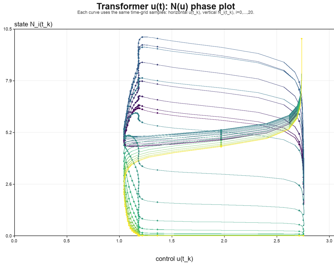
Figure 2. N(u) phase plot using the state-control points (u(t_k), N_i(t_k)) for all state components.
