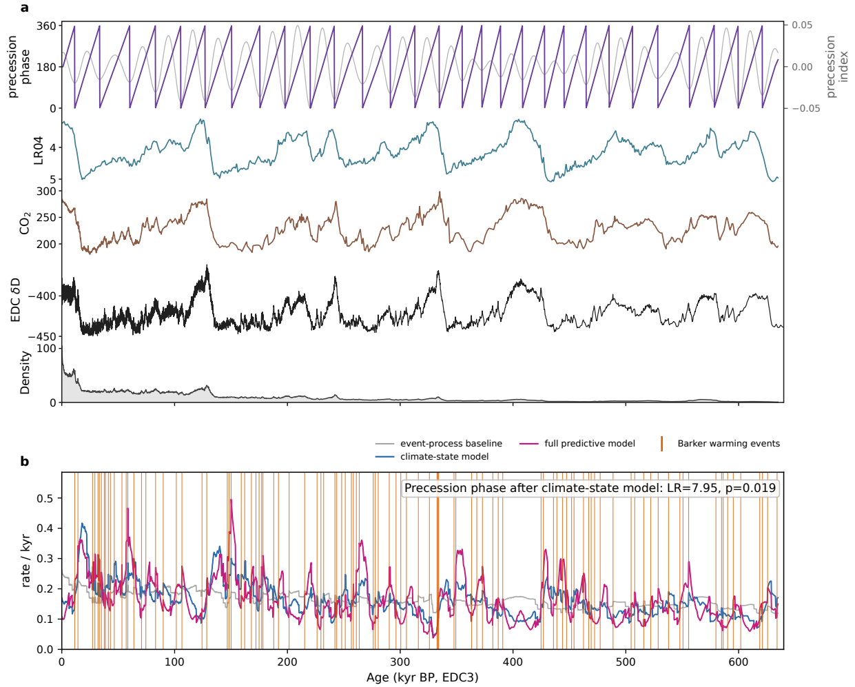
Figure S9: Barker EDC3 0–640 kyr inputs and fitted event rates. (a) Stacked input series: precession phase and raw precession index ( Laskar et al. , 2004), LR04 ( Lisiecki and Raymo , 2005), atmospheric CO 2 ( Bereiter et al. , 2015), EDC δD ( Jouzel et al. , 2007), and local EDC sampling density estimated from the EDC record used for the sampling-resolution term. (b) Fitted Barker warming-event rates for the event-process baseline, climate-state model, and full predictive model; vertical lines mark Barker variable-threshold warming events.
