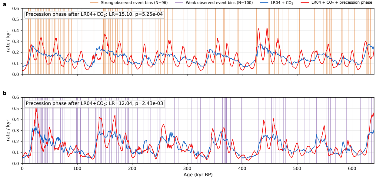
Figure S3: Climate-state and precession-phase fitted event rates without event-process controls. Fitted binned Poisson event rates from the LR04+CO 2 model and the LR04+CO 2 +precession-phase model are shown for (a) strong and (b) weak monsoon starts. Vertical lines mark observed event bins. This visualization omits same-type event history and sampling-resolution controls, so it is not the main reference model; it is included to show the slower climate-state rate modulation and the superposed precession-phase structure more clearly. Text boxes report likelihood-ratio tests for adding the two precession-phase terms to the LR04+CO 2 model. LR04, CO 2 , and precession phase are from Lisiecki and Raymo (2005), Bereiter et al. (2015), and Laskar et al. (2004), respectively.
