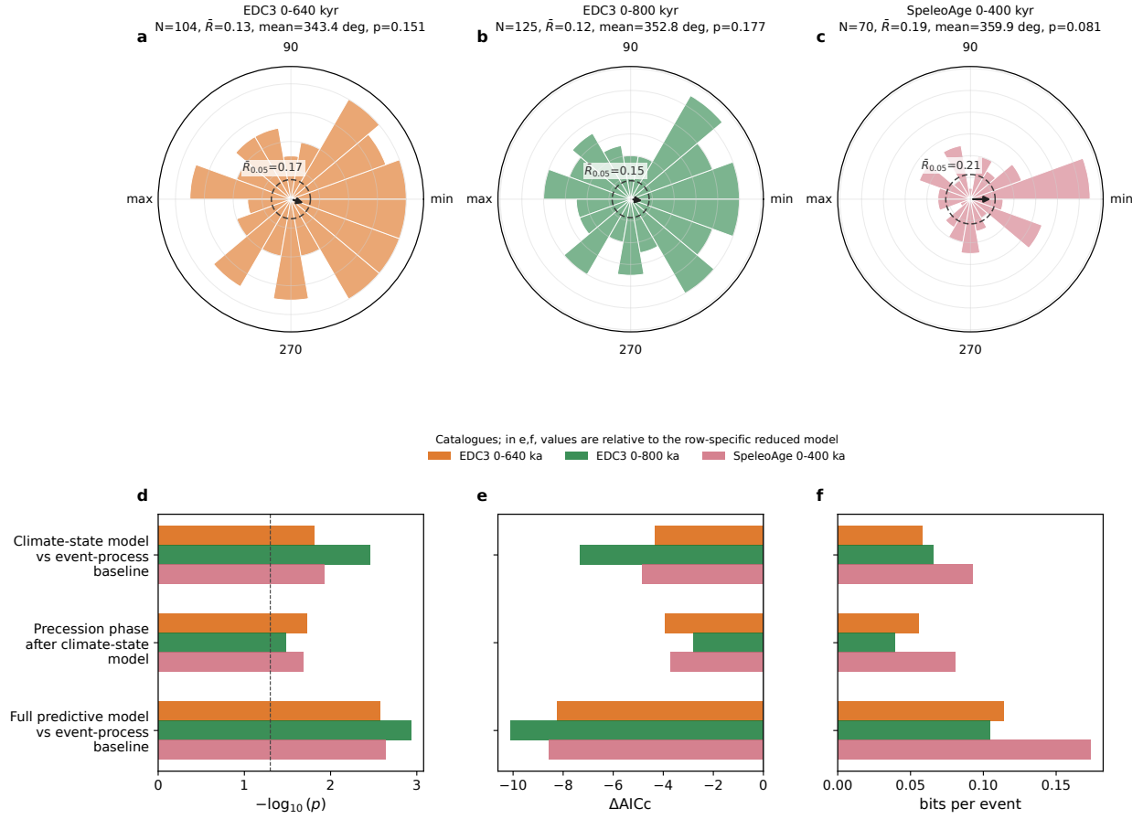
Figure S8: Barker et al. D-O warming catalogue sensitivity. (a–c) Precession-phase Rayleigh tests for the Barker et al. (2011) variable-threshold D-O warming catalogue under three age/support choices; arrows show the mean resultant direction and dashed circles mark the p = 0.05 threshold. (d) Nested likelihood-ratio tests shown as -\log_{10}(p) ; the dashed line marks p = 0.05 . (e) \Delta AICc , defined as full minus reduced model for each row; negative values favour the fuller model. (f) Predictive-information gain in bits per event for the same full-versus-reduced comparison. For each row, the reduced model is specified by the “after” phrase: the EDC event-process baseline for the climate-state model, the Barker climate-state model for precession phase, and the EDC event-process baseline for the full predictive model.
