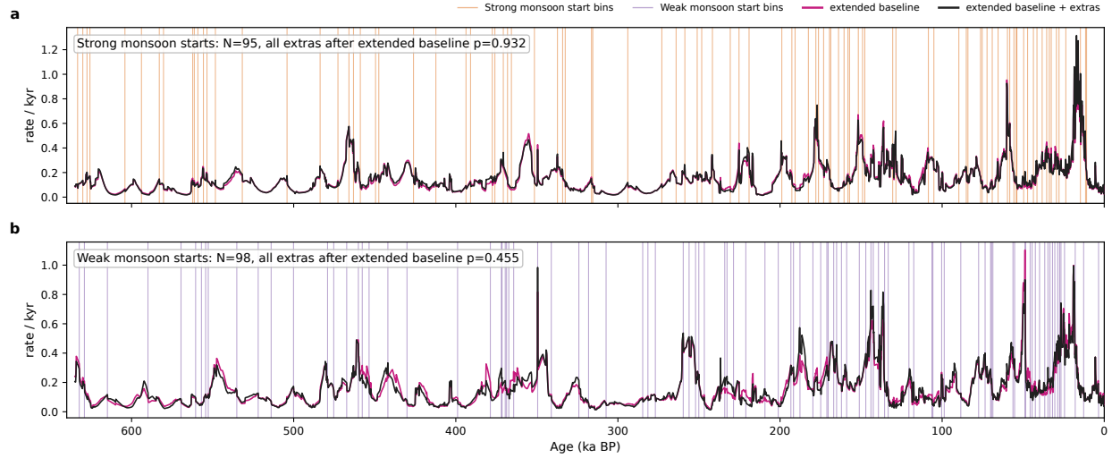
Figure S6: Extended-forcing fitted event rates. Fitted event rates from the predictive-information models are shown for (a) strong and (b) weak monsoon starts. Vertical lines mark observed event bins. Magenta curves show the extended baseline, i.e., the full predictive model before adding extra forcings; black curves show the extended model after adding Antarctic temperature, obliquity, eccentricity, and 65°N summer-solstice insolation. The similar fitted rates and nonsignificant likelihood-ratio tests indicate that the extra forcings do not significantly improve the extended baseline.
