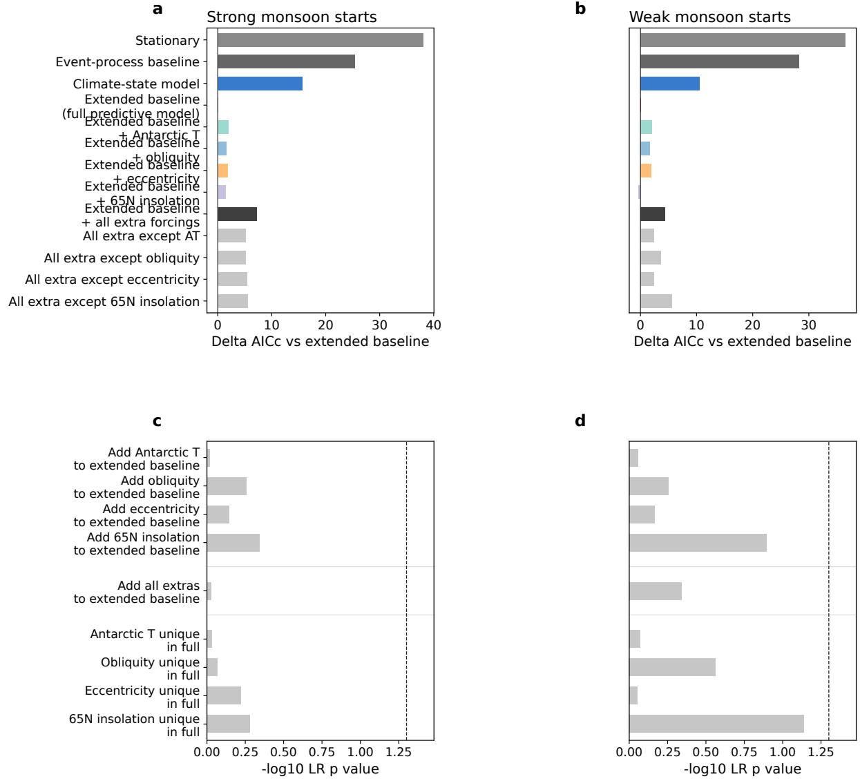
Figure S5: Additional-forcing sensitivity. Sensitivity of predictive-information models to additional forcings. (a,b) \Delta\text{AICc} for strong and weak monsoon starts, measured relative to the extended baseline, i.e., the full predictive model before adding extra forcings. (c,d) Nested likelihood-ratio tests for the extra forcings. Bars show -\log_{10}(p) , and the dashed line marks p = 0.05 ; bars to the left of this line are not significant. The three blocks test, from top to bottom, adding individual forcings to the extended baseline, adding all extra forcings jointly, and the unique contribution of each forcing within the full extended model.
