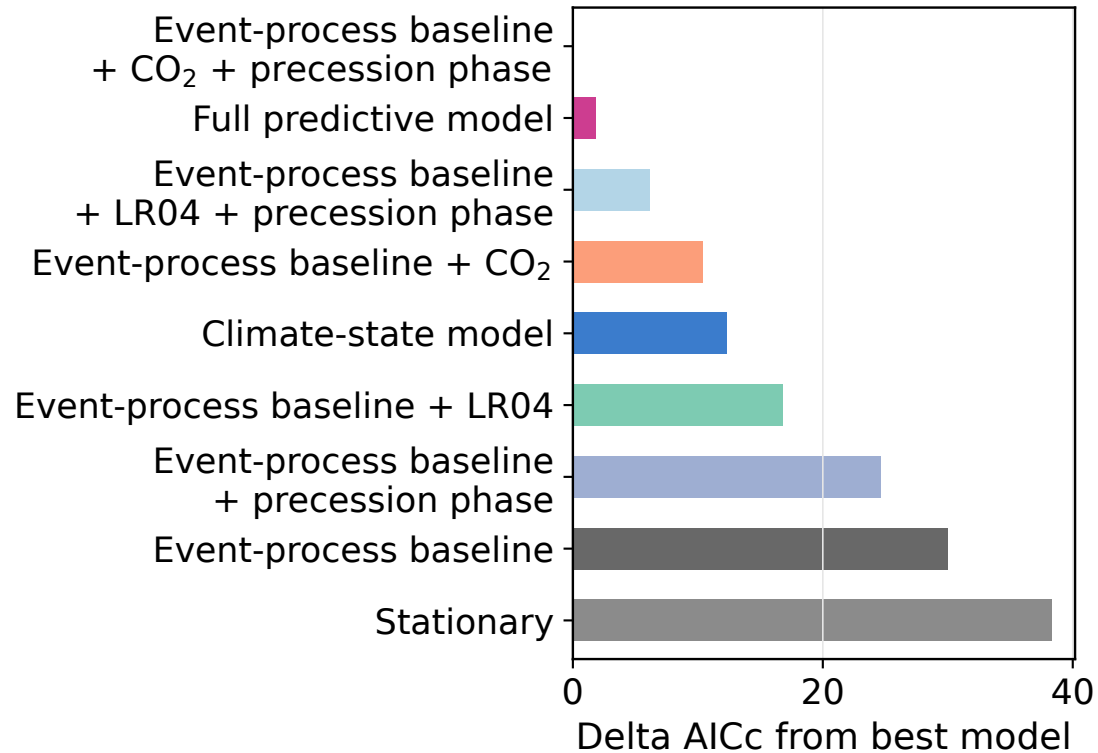
b Weak monsoon starts
