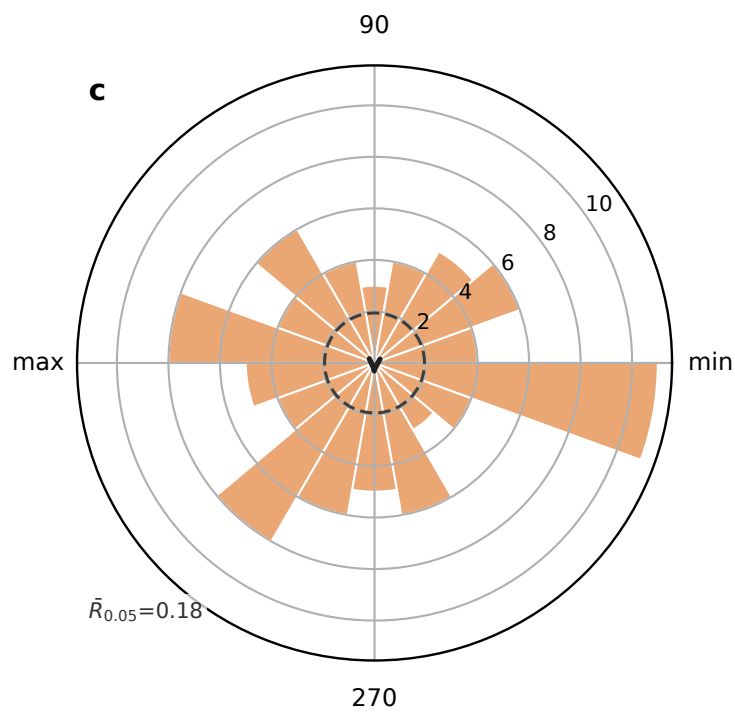
Strong monsoon starts N=96, \bar{R}=0.06 , p=0.682
