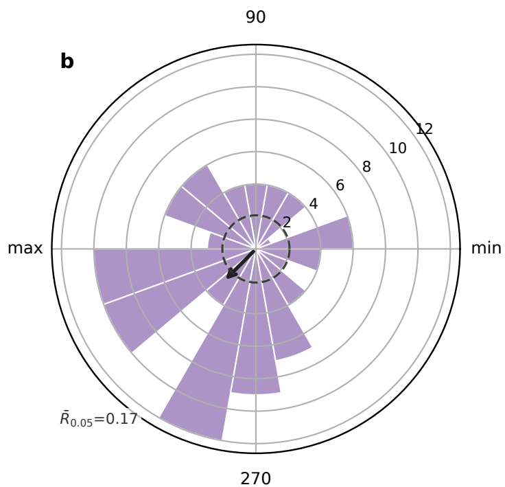
Weak monsoon starts N=100, \bar{R}=0.24 , p=0.003
