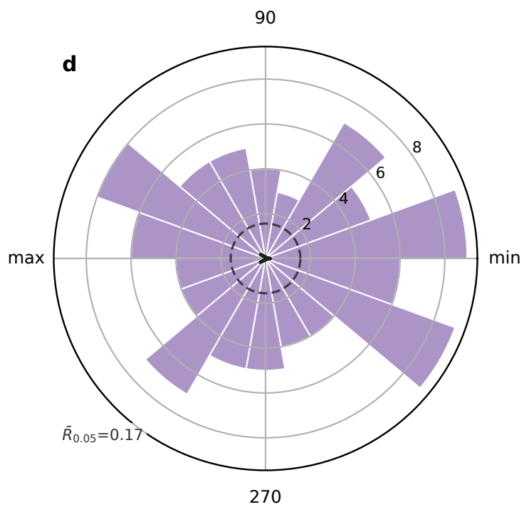
Weak monsoon starts N=100, \bar{R}=0.05 , p=0.760
