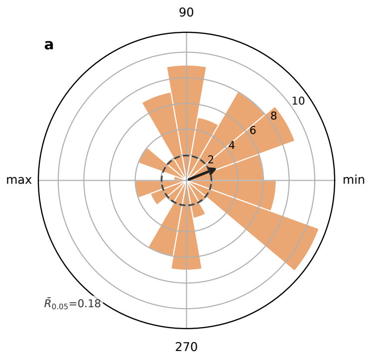
Strong monsoon starts N=96, \bar{R}=0.25 , p=0.002
