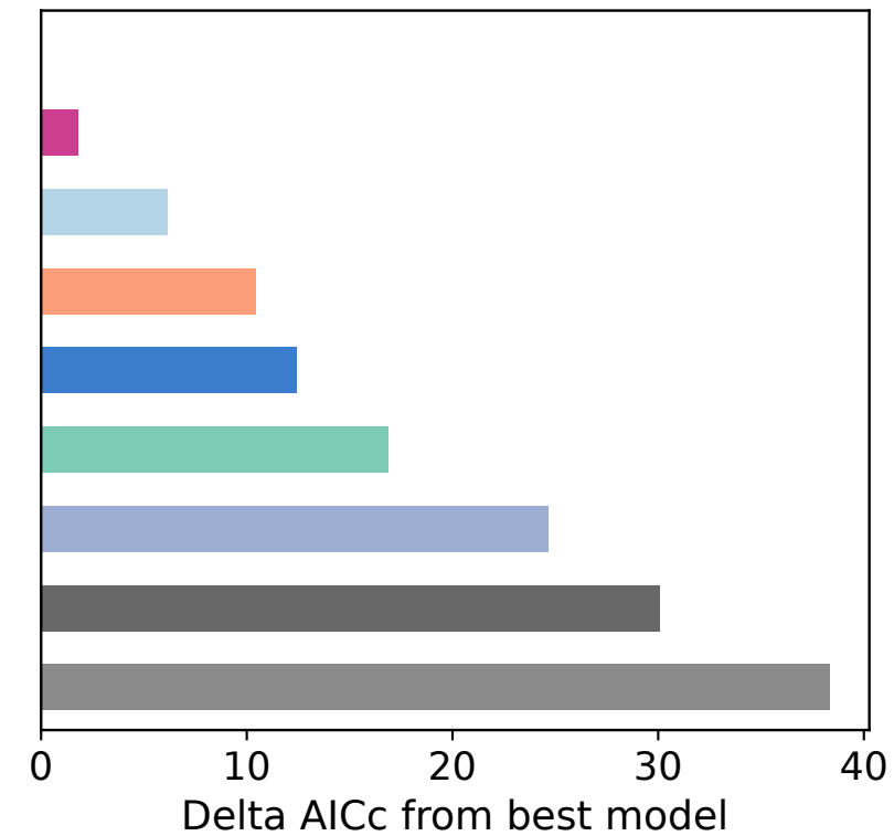
b Weak monsoon starts
