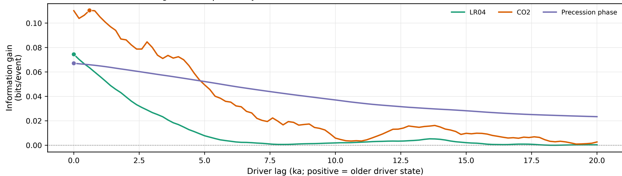
Weak monsoon starts: single drivers | Y history
