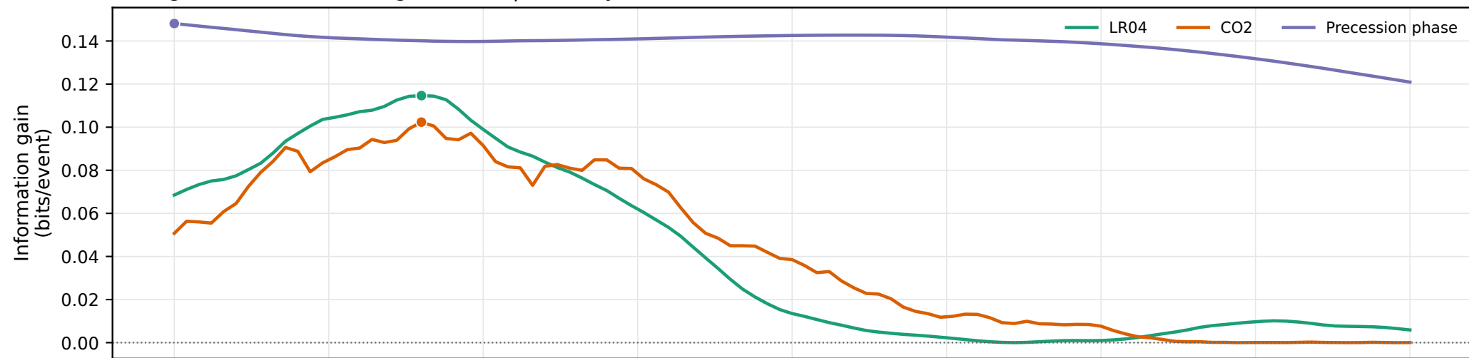
Strong monsoon starts: single drivers | Y history
