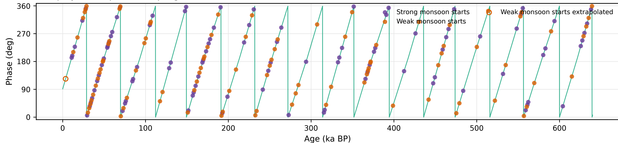
Obliquity: event phase sampling
