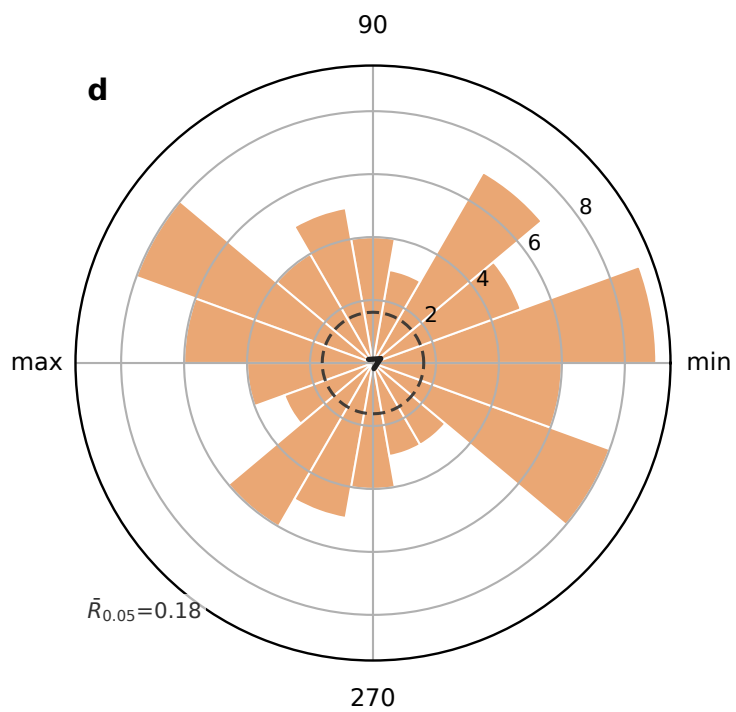
Obliquity Weak monsoon starts N=93, \bar{R}=0.07 , p=0.632
