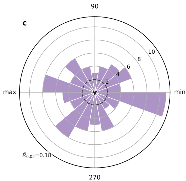
Obliquity Strong monsoon starts N=96, \bar{R}=0.06 , p=0.682
