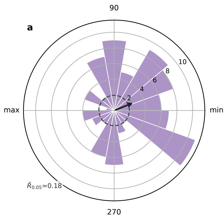
Precession index Strong monsoon starts N=96, \bar{R}=0.25 , p=0.002
