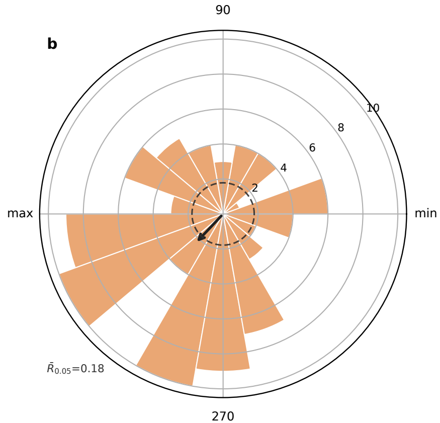
Precession index Weak monsoon starts N=94 , \bar{R}=0.23 , p=0.005
