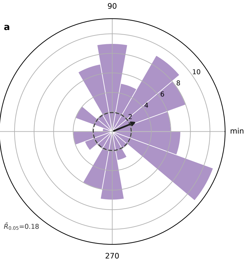
Precession index Strong monsoon starts N=96 , \bar{R}=0.25 , p=0.002
