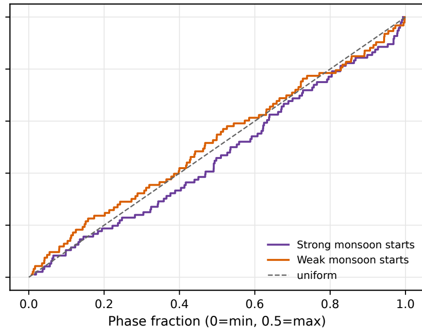
Obliquity phase ECDF
