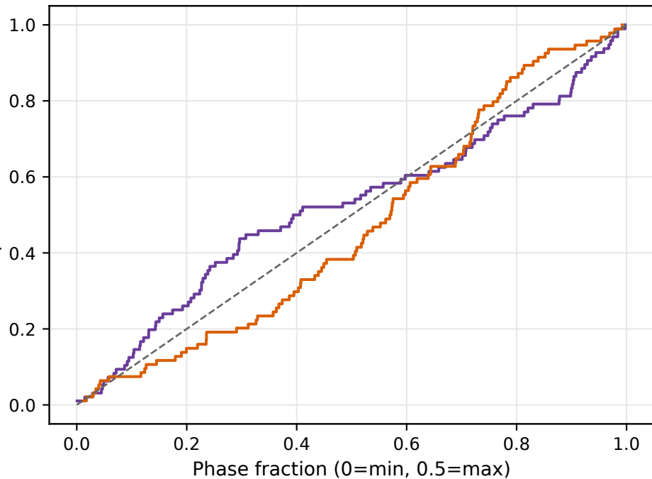
Precession index phase ECDF
