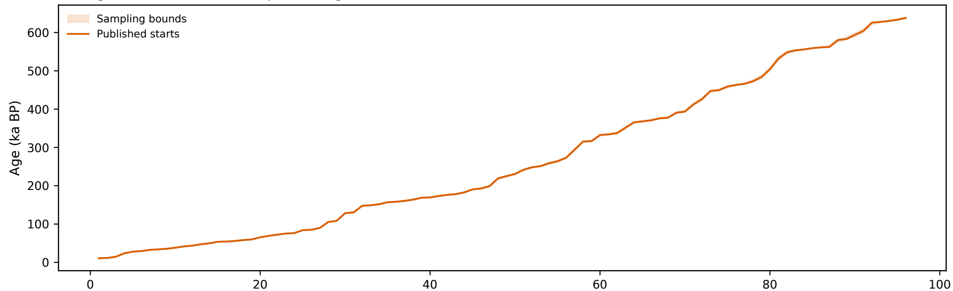
Weak monsoon starts: rank-preserving truncated Gaussian bounds
