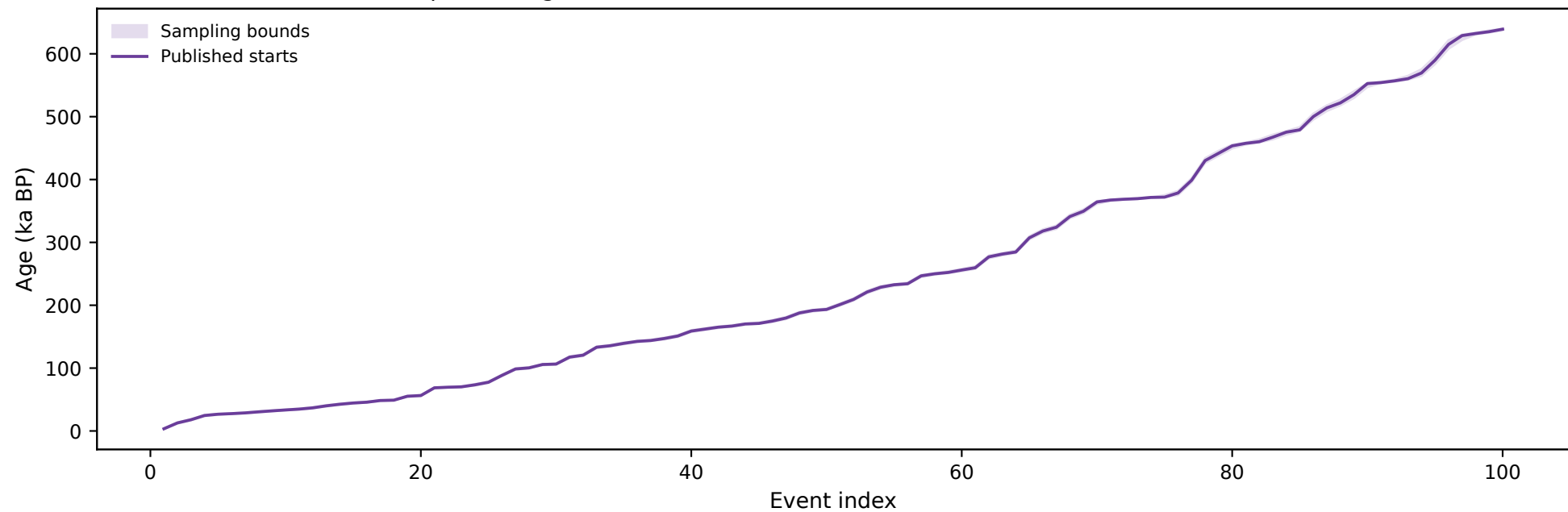
Weak monsoon starts: rank-preserving truncated Gaussian bounds
