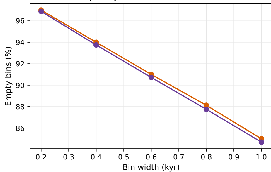
Event-count sparsity
