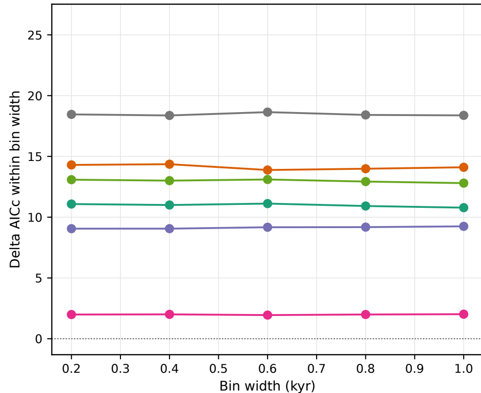
Strong monsoon starts
