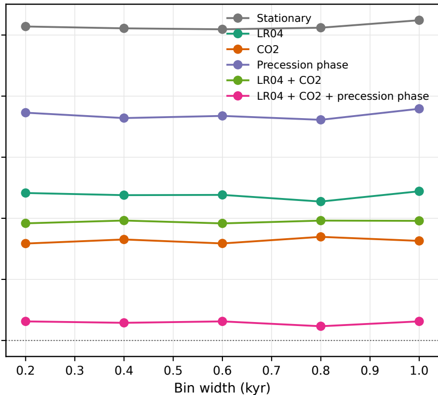
Weak monsoon starts
