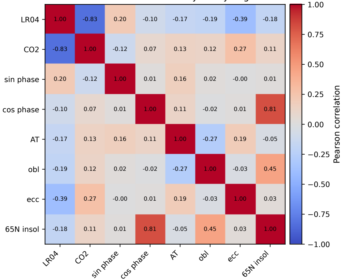
Predictor correlation on the 0.2 kyr analysis grid
