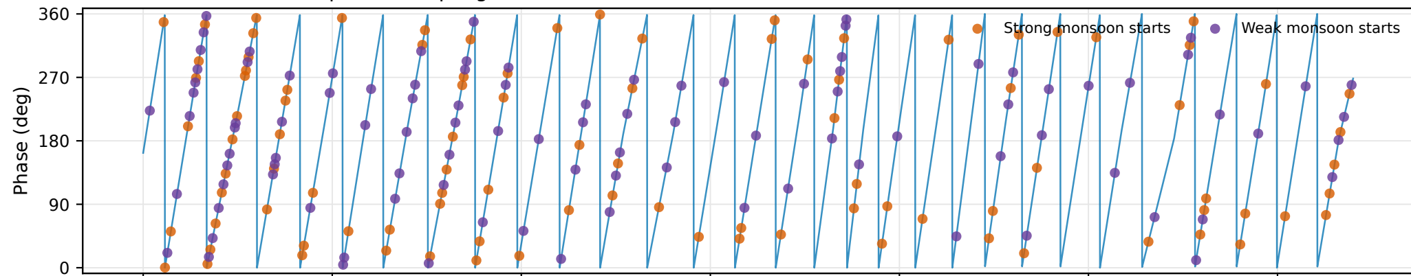
Precession index: event phase sampling
