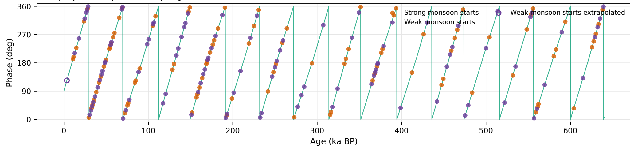
Obliquity: event phase sampling
