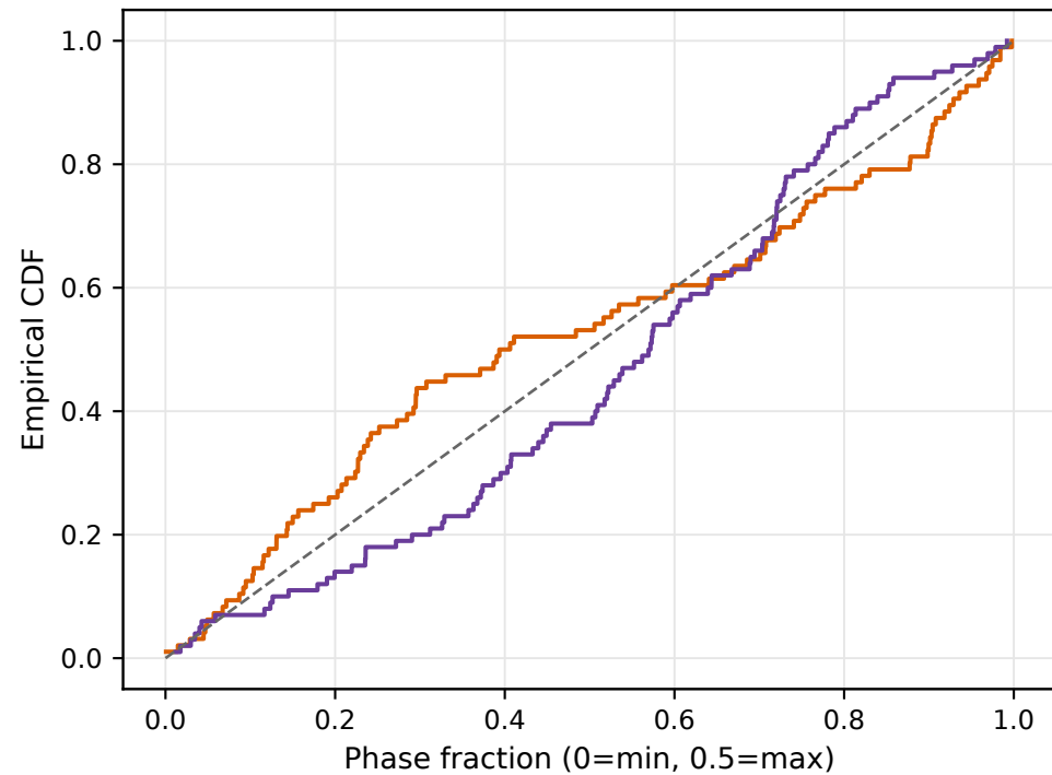
a Precession index phase ECDF
