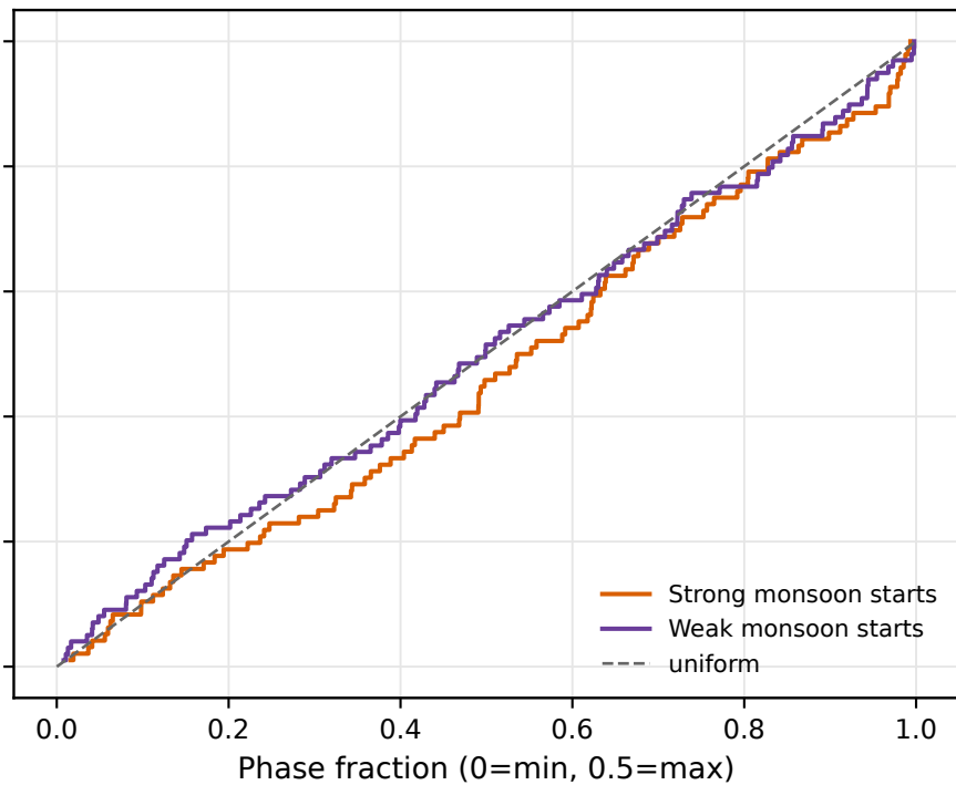
b Obliquity phase ECDF
