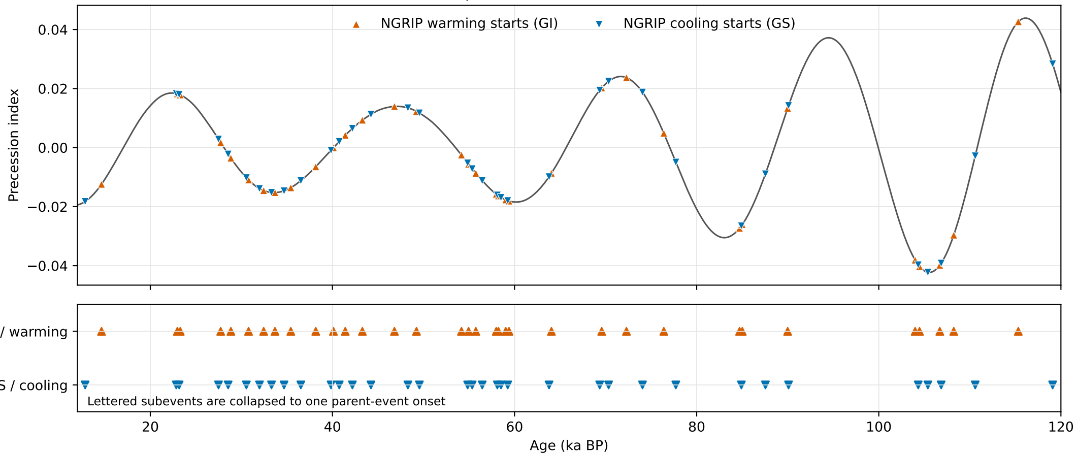
Rasmussen et al. (2014) main GI/GS starts and precession
