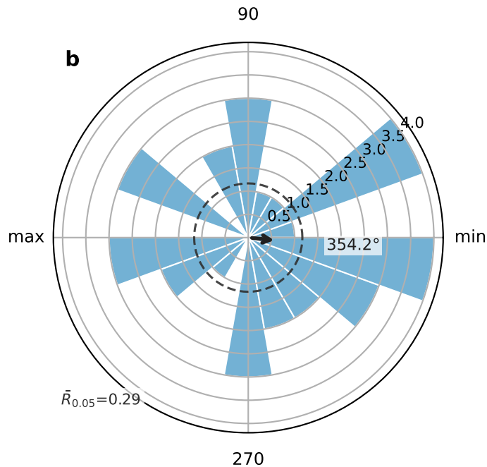
NGRIP cooling starts (GS) N=35, \bar{R}=0.16 , p=0.407
