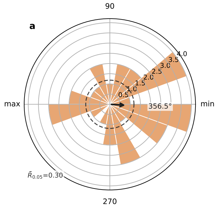
NGRIP warming starts (GI) N=34, \bar{R}=0.21 , p=0.224
