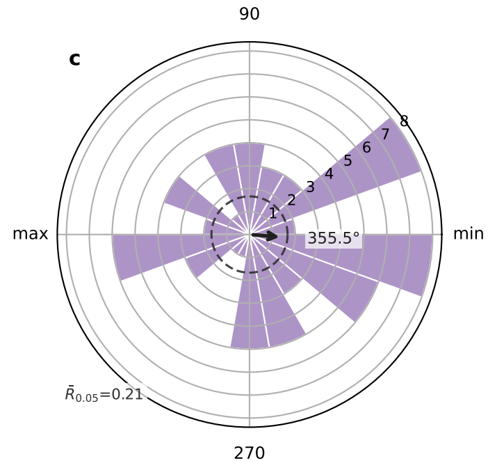
All NGRIP transitions (GI + GS) N=69, \bar{R}=0.19 , p=0.093
