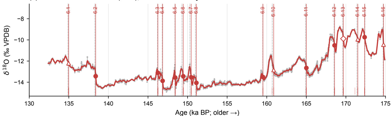
(c) Huagapo — Burn et al. (2019); Gaussian \sigma = 100 yr
