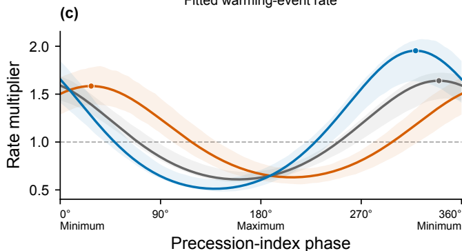
Fitted warming-event rate
