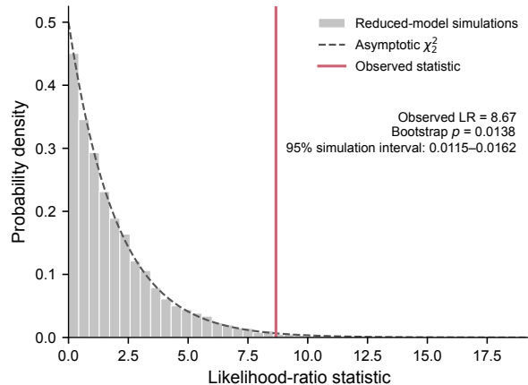
(b) Barker 2011
