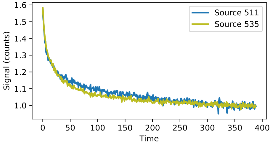
Median curves of sources 511 & 535
