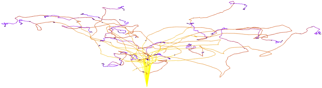
Figure 10: Example of electron tracks in a water medium. The track color shows changes in the electron energy.
