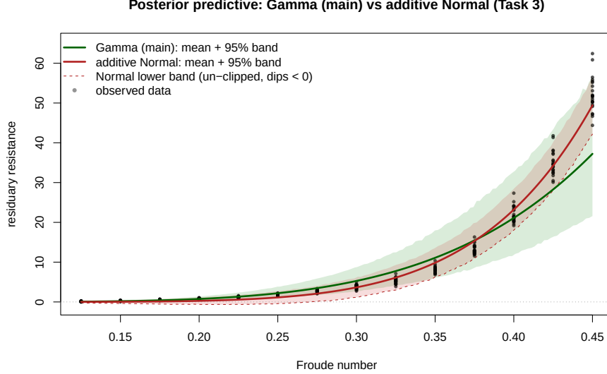
Figure 3: Posterior-predictive bands of the Gamma main model (green) and the additive-Normal sensitivity fit (red) on the original resistance scale, with observed data. The additive Normal’s mean curve is steeper and its un-clipped lower band (dashed) dips below zero at low Froude, whereas the Gamma’s lower band stays non-negative.
