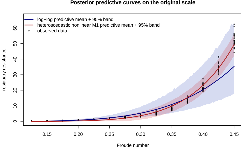
Figure 4: Posterior predictive curves on the original resistance scale. The blue band is the log-log model after back-transformation, and the red band is the heteroscedastic nonlinear M1 model. Points are the observed yacht resistance data.
