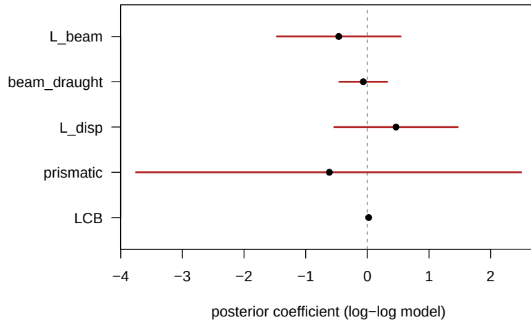
Figure 10: Posterior means and 95% credible intervals of the five hull-geometry coefficients in the log-log model. Every interval straddles zero (dashed line), indicating that no single form factor is resolved once the Froude number is accounted for.
