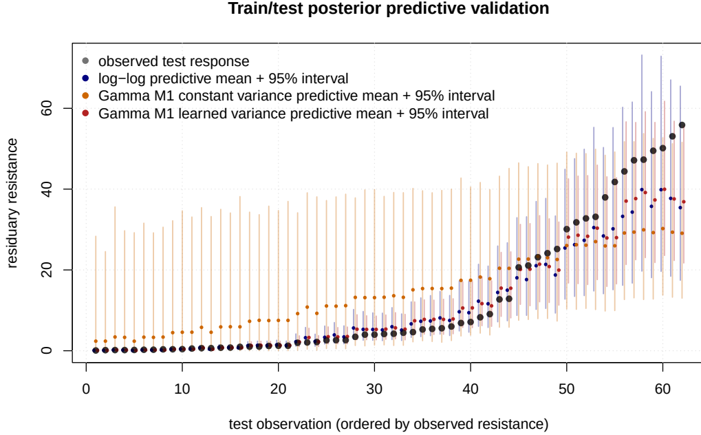
Figure 6: Train/test posterior predictive validation on the held-out rows. The black points are observed test responses ordered by resistance. Coloured points show posterior predictive means, and vertical intervals show the corresponding 95% posterior predictive bands for the log-log model, the constant-variance Gamma M1 model, and the learned-variance Gamma M1 model.
