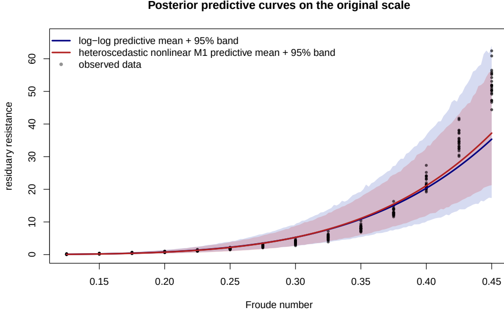
Figure 4: Posterior predictive curves on the original resistance scale. The blue band is the log-log model after back-transformation, and the red band is the heteroscedastic nonlinear M1 model. Points are the observed yacht resistance data.
