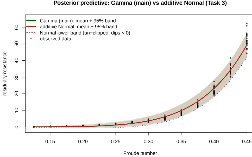
Figure 3: Posterior-predictive bands of the Gamma main model (green) and the additive-Normal sensitivity fit (red) on the original resistance scale, with observed data. The additive Normal’s mean curve is steeper and its un-clipped lower band (dashed) dips below zero at low Froude, whereas the Gamma’s lower band stays non-negative.
