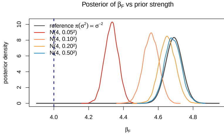
Figure 11: Posterior density of the Froude exponent \beta_F under the independent informative priors \mathcal{N}(4, \tau^2) of increasing strength (coloured, Gibbs samples) and under the reference prior (grey, closed-form Student- t ). The dashed blue line marks the physical value \beta_F = 4 . Tightening the prior toward 4 shifts the posterior only modestly; the data keep it well above 4 unless the prior is unreasonably confident.
