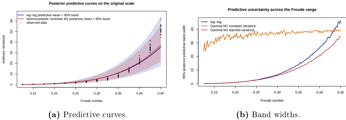
Figure 2: Posterior predictive comparison on the resistance scale. Left: fitted predictive bands and observed data. Right: interval width across Froude number.
