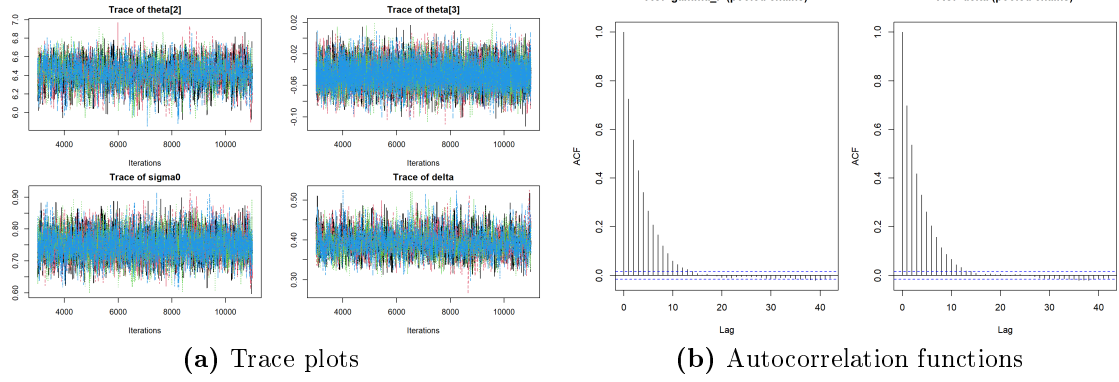
Figure A.6: Trace plots and autocorrelation functions for model M1; each colour represents a chain.
