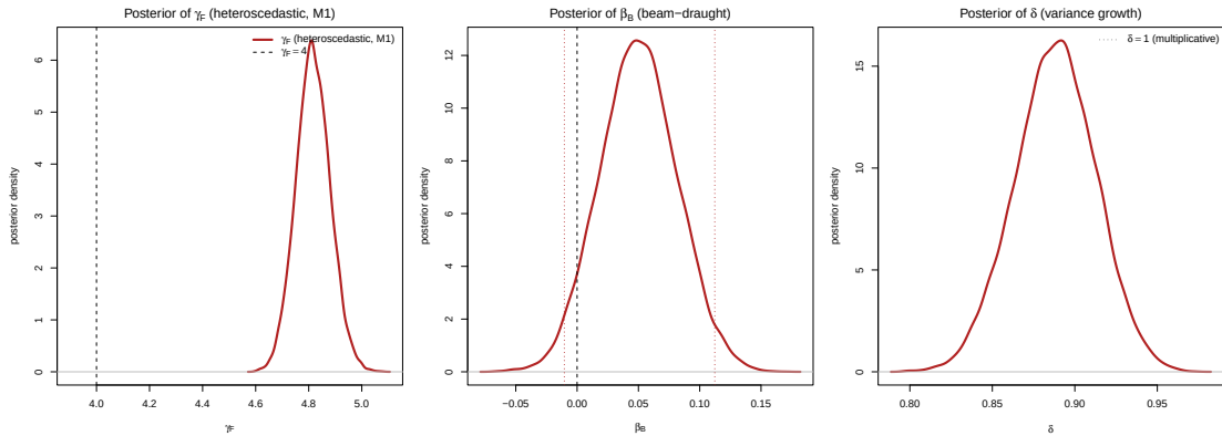
Figure 1: Marginal posteriors for the heteroscedastic nonlinear model M1 (Gamma likelihood). Left: the Froude exponent \gamma_F , with the dashed line at the physical value 4. Centre: the beam–draught coefficient \beta_B , with the dashed line at 0. Right: the variance-growth exponent \delta , with the multiplicative value \delta = 1 marked.
