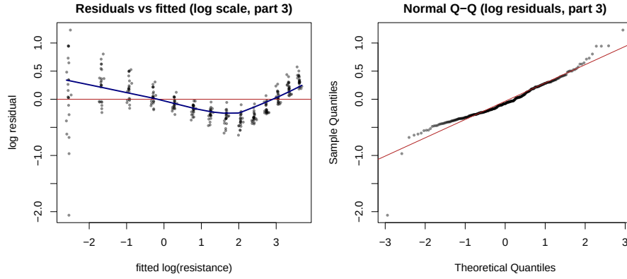
Figure A.9: Log-scale residual diagnostics for the nonlinear model M1, plotted on the same axes as the part-1 log-log diagnostics (Fig. A.3) for a like-for-like comparison. Left: log residuals \log y_i - \log \hat{\mu}_i versus the fitted log-resistance \log \hat{\mu}_i , with a LOWESS trend (navy). Right: Normal Q-Q plot of the log residuals. Because the learned variance is close to multiplicative ( \delta \approx 0.9 ), the M1 residuals are nearly homoscedastic on the log scale as well, mirroring the log-log fit; this is the log-lens counterpart of the agreement between \gamma_F \approx 4.82 and the log-log exponent \beta_F \approx 4.69 . The original-scale diagnostics (Fig. A.8) remain the proper goodness-of-fit check for M1.
