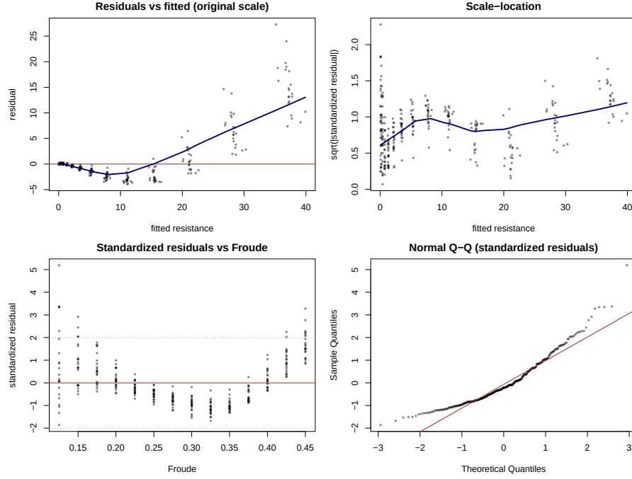
Figure A.8: Original-scale residual diagnostics for the heteroscedastic nonlinear model M1, with each residual standardized by its own fitted standard deviation \hat{\sigma}_i = \hat{\sigma}_0 \hat{\mu}_i^\delta . Top left: raw residuals versus fitted resistance with a LOWESS trend (navy); the spread still fans out, the heteroscedasticity that the variance model must absorb. Top right: scale–location plot, \sqrt{|\text{standardized residual}|} versus fitted value; the roughly flat trend shows the learned variance function \sigma_i = \sigma_0 \mu_i^\delta removes the funnel. Bottom left: standardized residuals versus the Froude number with the \pm 2 reference band; no remaining trend against the physical driver. Bottom right: Normal Q–Q plot of the standardized residuals. After standardization the spread is close to unity and about 95% of points lie within \pm 2 , confirming that learning the variance corrects the heteroscedasticity.
