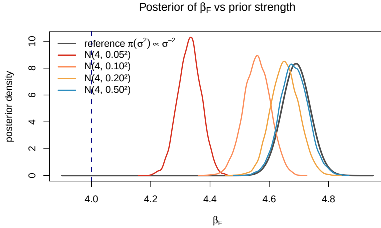
Figure A.5: Posterior density of the Froude exponent \beta_F under the independent informative priors \mathcal{N}(4, \tau^2) of increasing strength (coloured, Gibbs samples) and under the reference prior (grey, closed-form Student- t ). The dashed blue line marks the physical value \beta_F = 4 . Tightening the prior toward 4 shifts the posterior only modestly; the data keep it well above 4 unless the prior is unreasonably confident.
