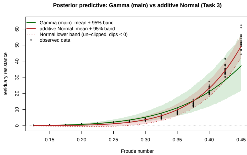
Figure A.7: Posterior-predictive bands of the Gamma main model (green) and the additive-Normal sensitivity fit (red) on the original resistance scale, with observed data. The additive Normal’s mean curve is steeper and its un-clipped lower band (dashed) dips below zero at low Froude, whereas the Gamma’s lower band stays non-negative.
