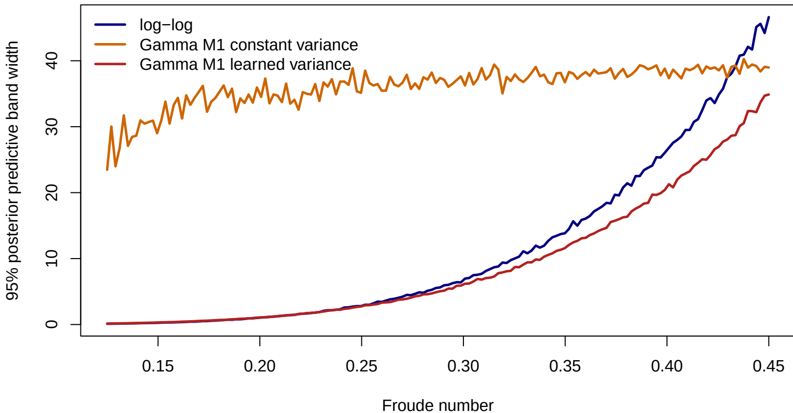
Predictive uncertainty across the Froude range
